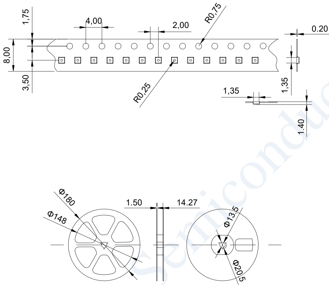
Figure 24 Package Specification
