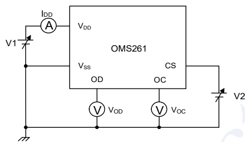
Figure 4 (Test Circuit 2)
