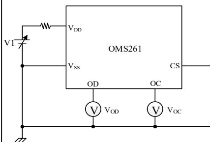
Figure 3 (Test Circuit 1)
