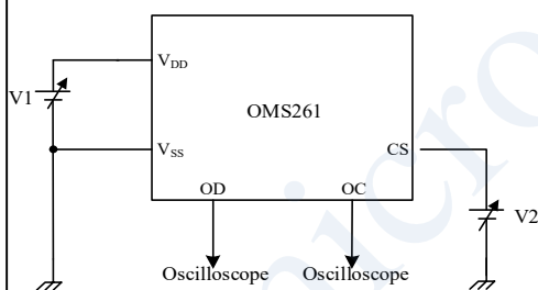
Figure 7 (Test Circuit 5)
